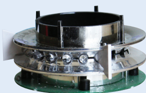
Partitioning of the Sealite LED reflector allows the lanterns to meet regulatory requirements
